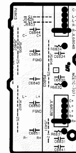
SPEAKER TERMINAL A PC BOARD
