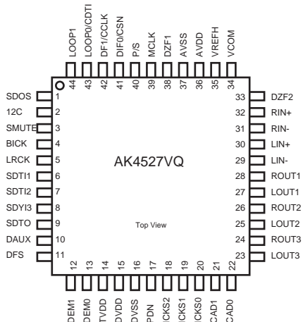
Pin Layout
