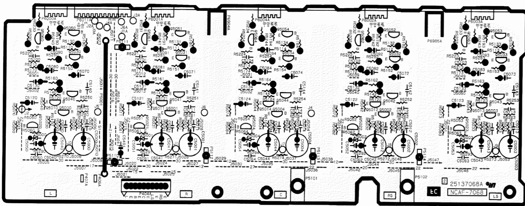
POWER AMPLIFIER A PC BOARD
