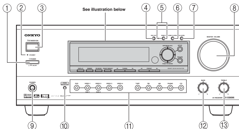
Front panel
