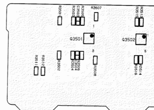
SOLDERING SIDE
