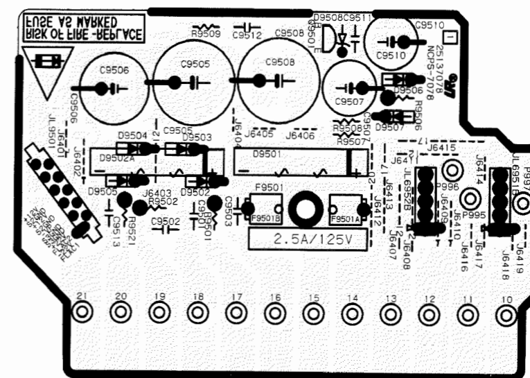
REGULATOR CIRCUIT PC BOARD
