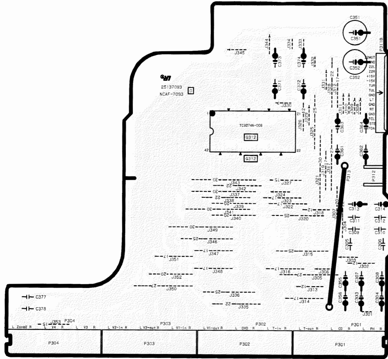
COMPONENT SIDE
