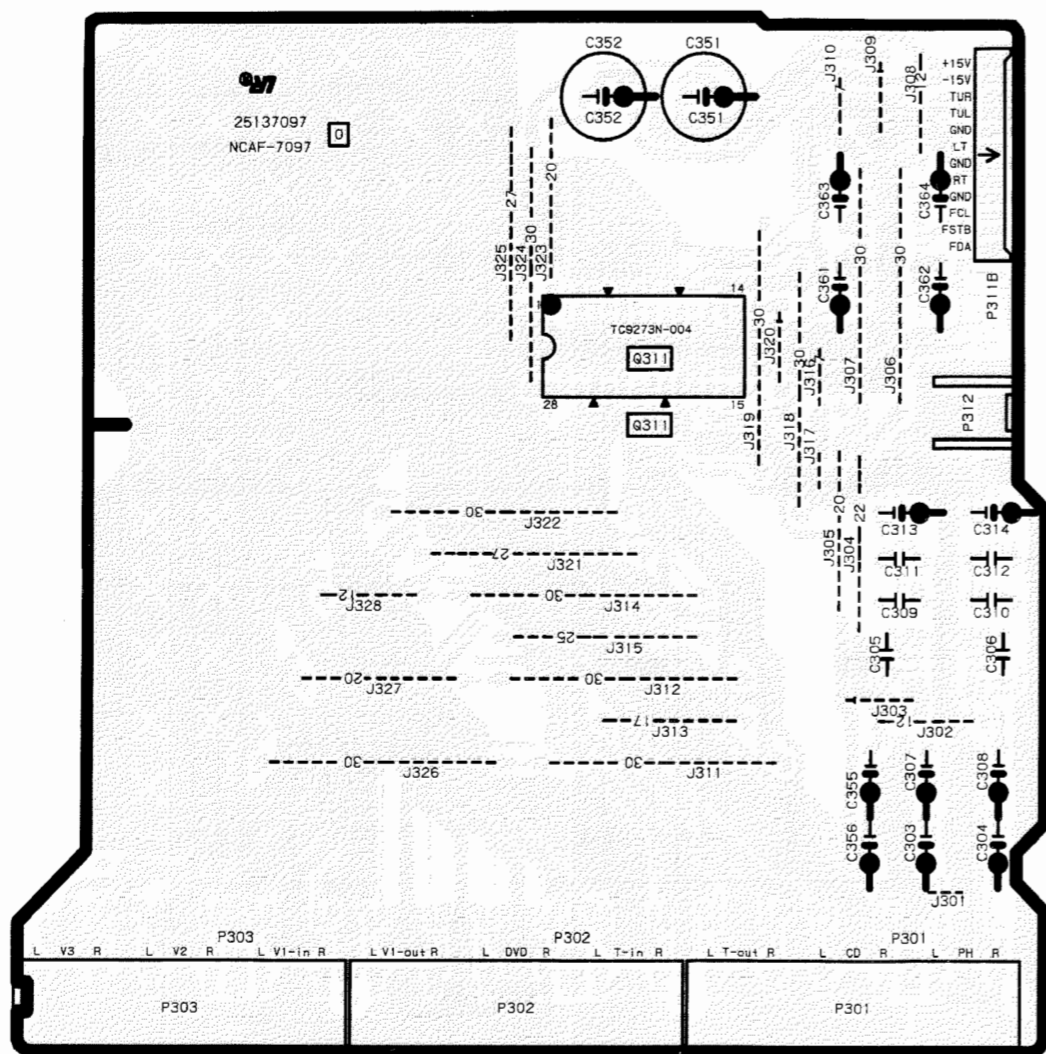
COMPONENT SIDE
