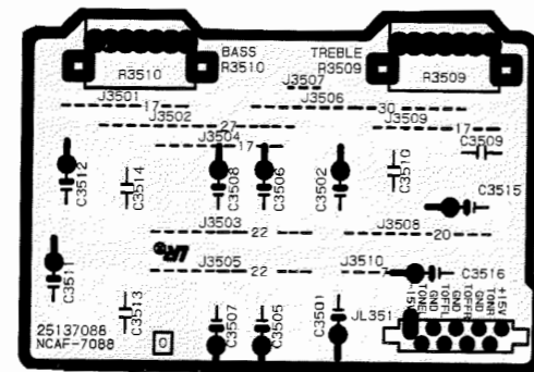
COMPONENT SIDE
