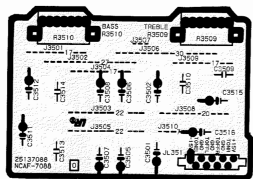
COMPONENT SIDE
