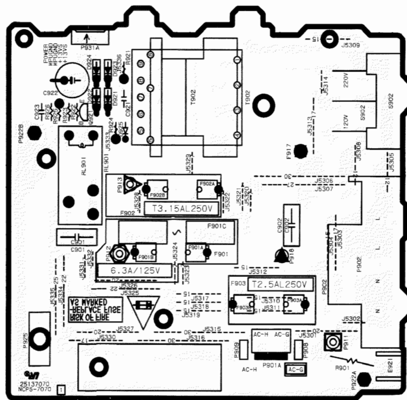
PRIMARY CIRCUIT PC BOARD
