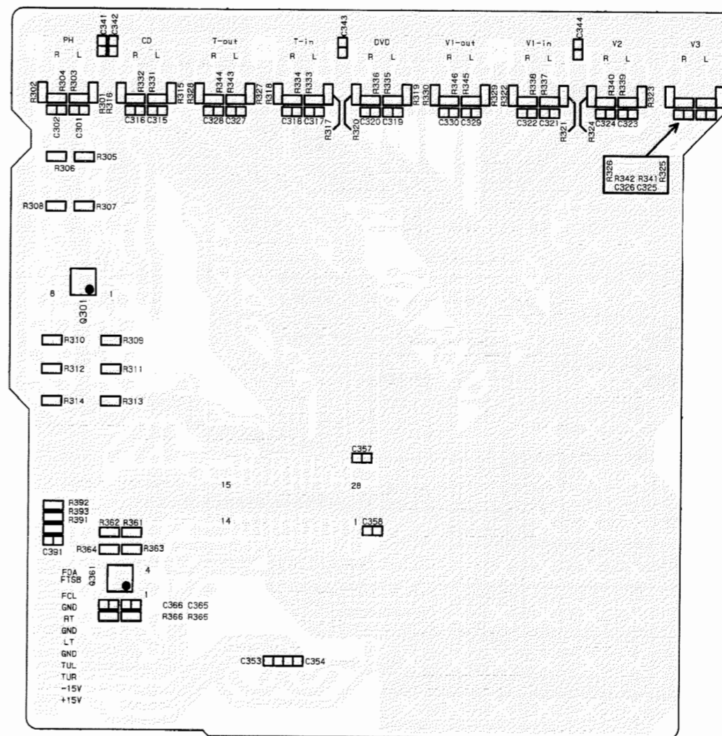
SOLDERING SIDE
